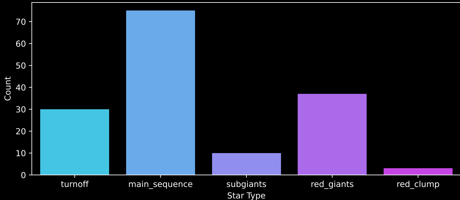
APOGEE DR17 Field: [SMC12] Count plot of Star Type
