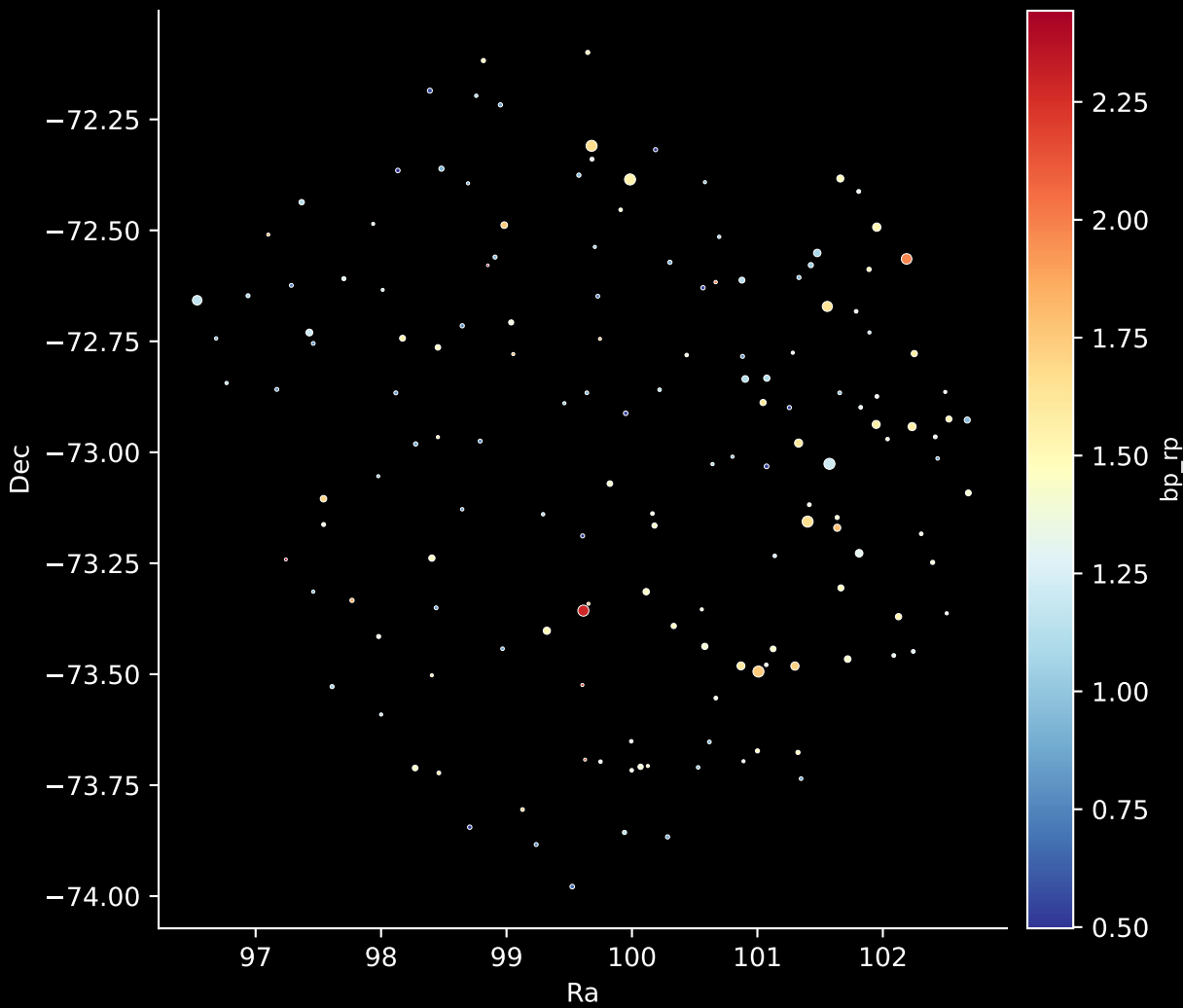
APOGEE DR17 Field: [SMC12] Stars: 155
