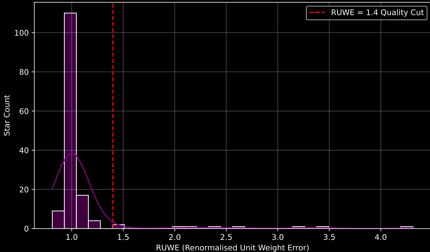
GAPOGEE DR17 Field [SMC12] RUWE Distribution (n= 149)
