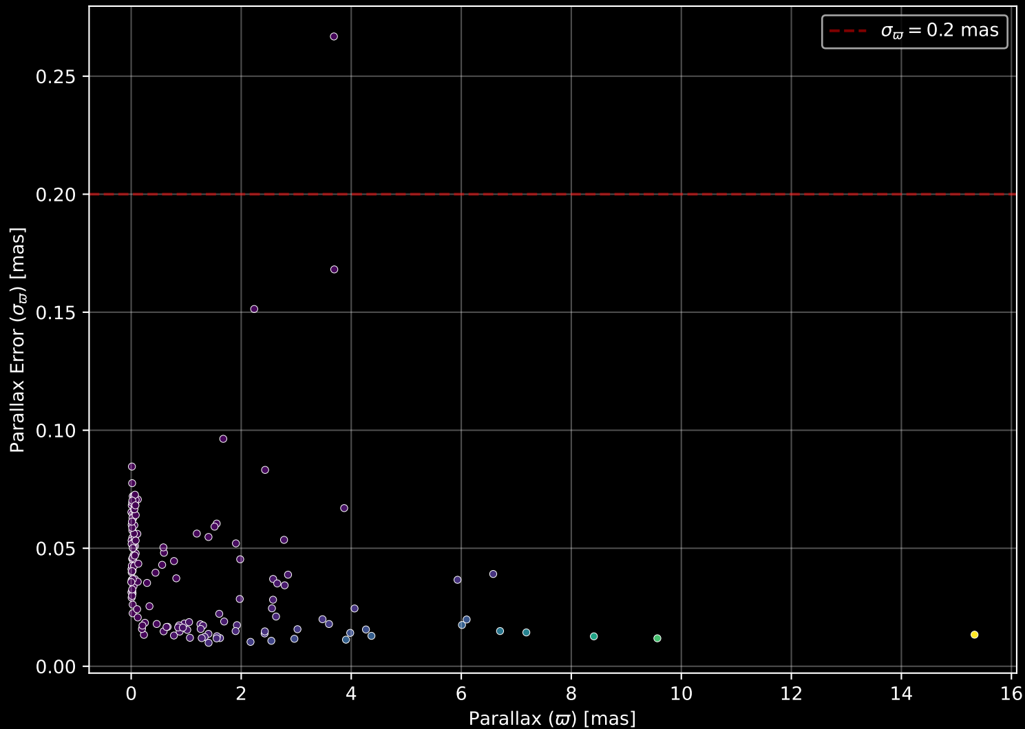
APOGEE DR17 Field: [SMC12] Parallax Quality (n= 155)
