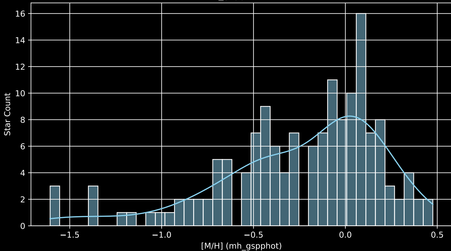
APOGEE DR17 Field: [SMC12 [M/H] (mh_gspphot) (n= 152)
