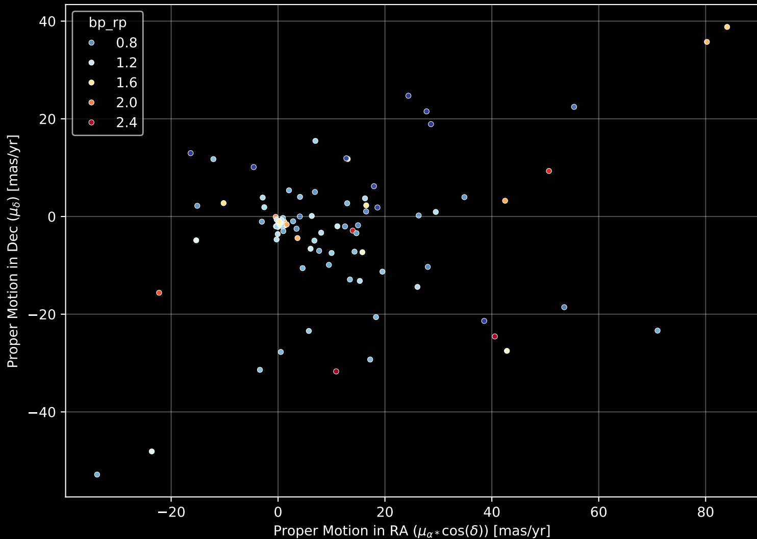
APOGEE DR17 Field: [SMC12] Proper Motion Diagram (n= 155)
