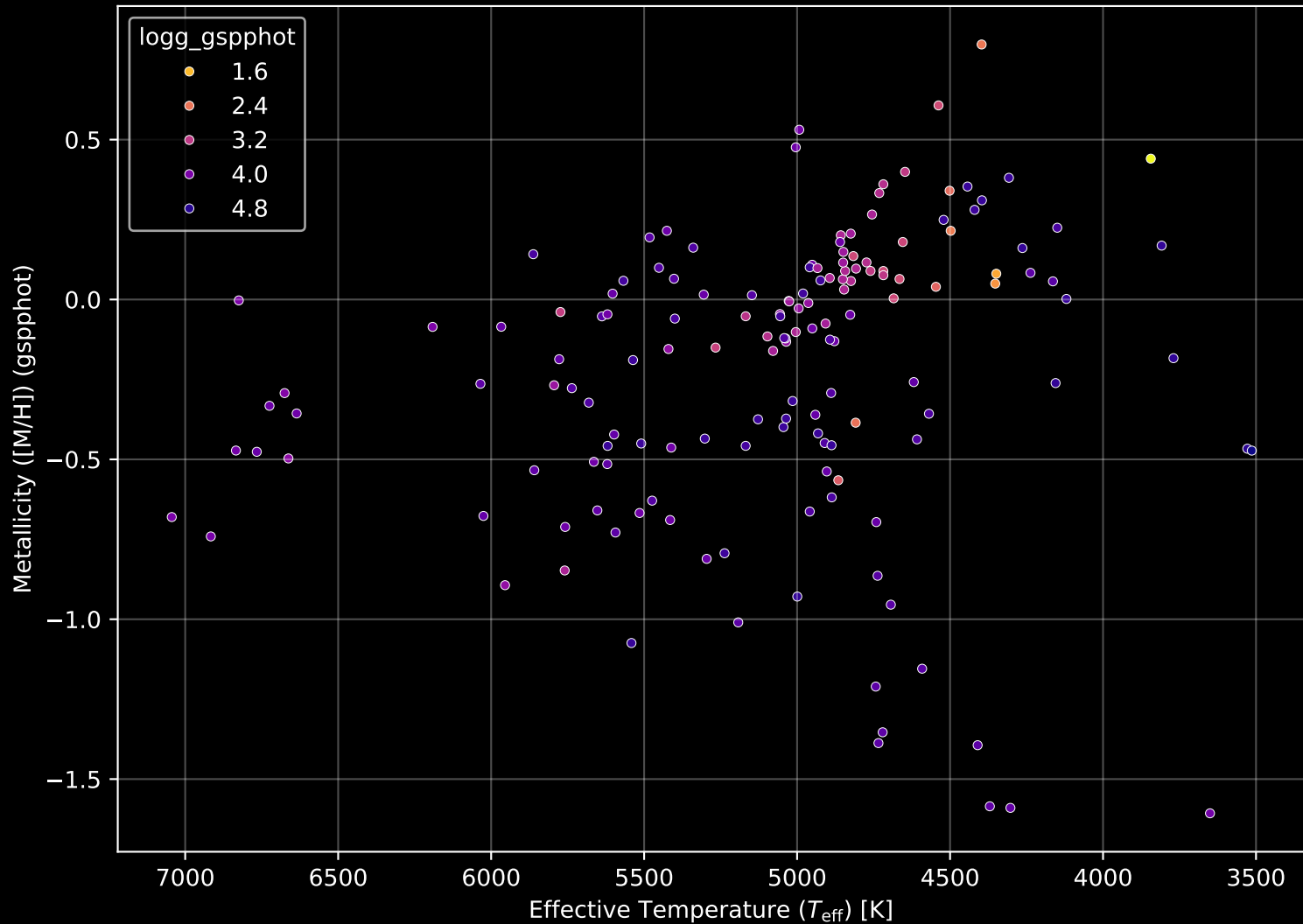
APOGEE DR17 Field: [SMC12] Stellar Population Parameters (n= 155)
